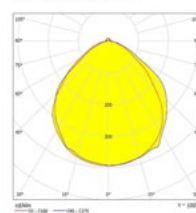
Luminance Distribution
