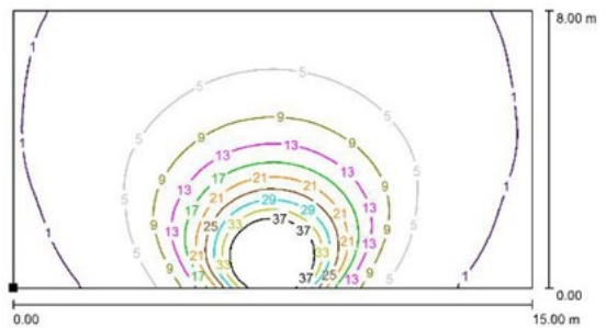
Illumination Curve
